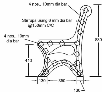
Reinforcement Detail of Leg (Isometric View)
