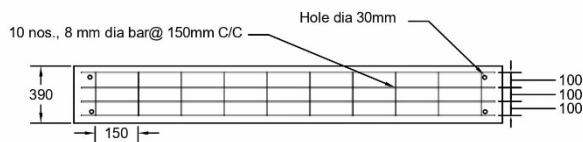
Reinforcement Plan of Top Plank (1510mm x 390mm x 70mm)
