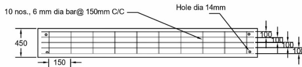
Reinforcement Plan of Bottom Plank (1520mm x 450mm x 70mm)
