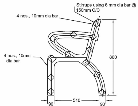
Reinforcement Detail of Leg
