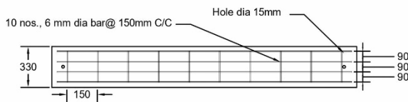
Reinforcement Plan of Top Plank (1520mm x 330mm x 70mm)
