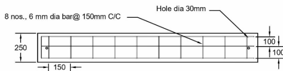
Reinforcement Plan of Top Plank (1360mm x 250mm x 70mm)
