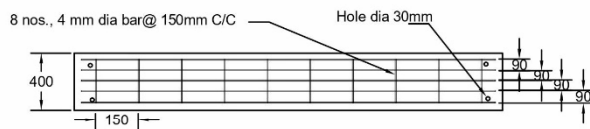
Reinforcement Plan of Bottom Plank (1360mm x 400mm x 70mm)
