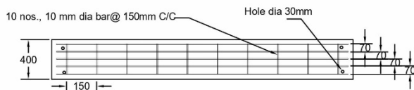
Reinforcement Plan of Bottom Plank (1510mm x 400mm x 70mm)
