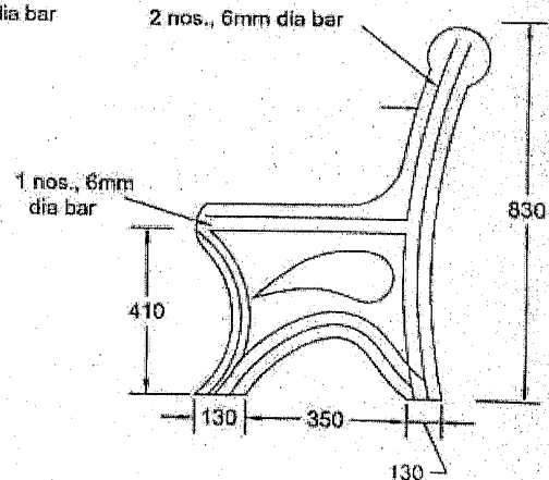
Reinforcement Detail of Leg (Isometric View)
