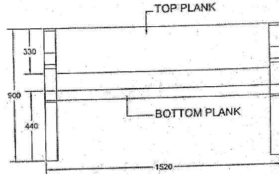
Front Elevation
