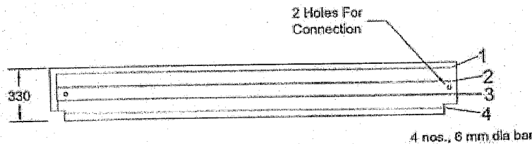
Reinforcement Plan of Top Plank (1500 mm X 330 mm)
