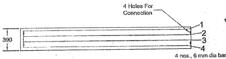
Reinforcement Plan of Top Plank (1510 mm X 390 mm)
