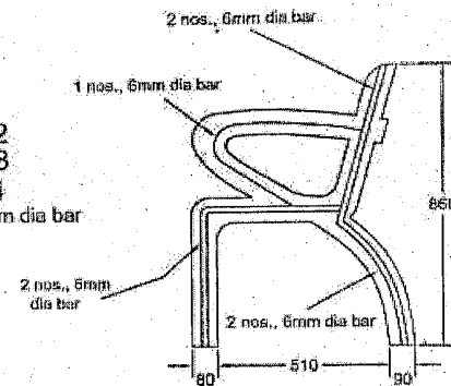
Reinforcement Detail of Leg
