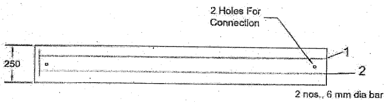
Reinforcement Plan of Top Plank (1360 mm X 250 mm)
