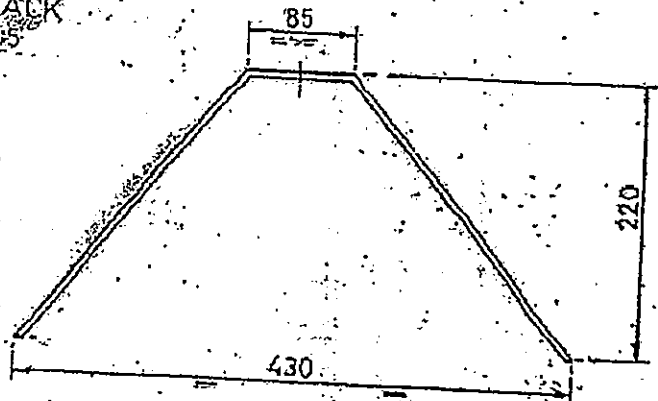
8 BACK TYNE SUPPORT SCALE-1:5
