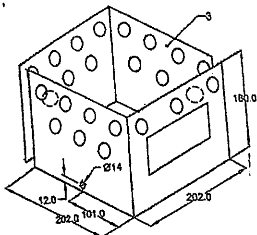
COMBUSTION CHAMBER
