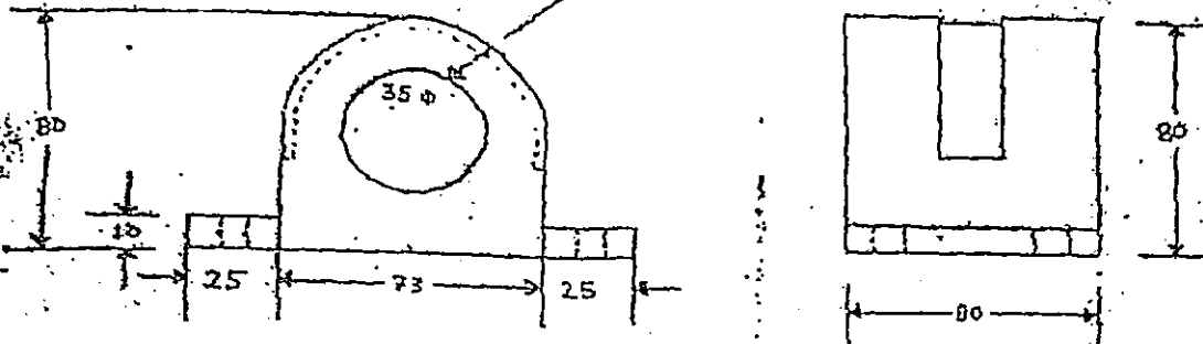
PLUMMER BLOCK
