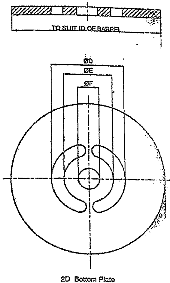
FIG. 2 DETAIL OF SOLID BIO-MASS COOKSTOVE DESIGN 'A' — (Concluded)
