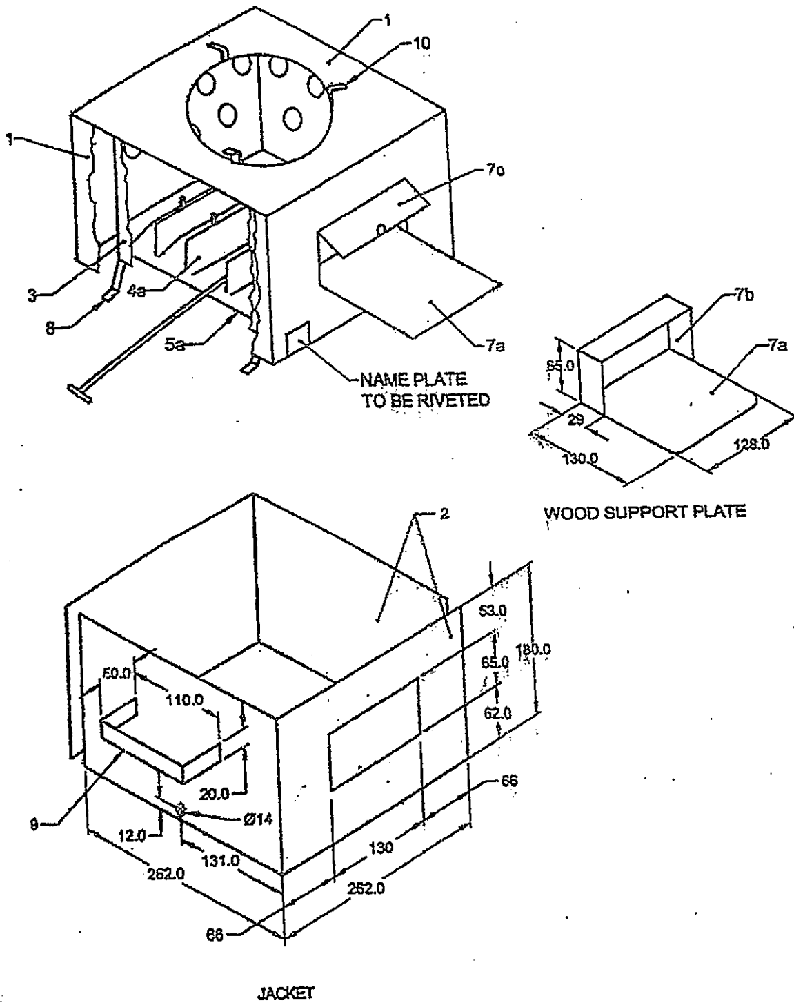
FIG. 3 SOLID BIO-MASS COOKSTOVE DESIGN 'B' — (Continued)
