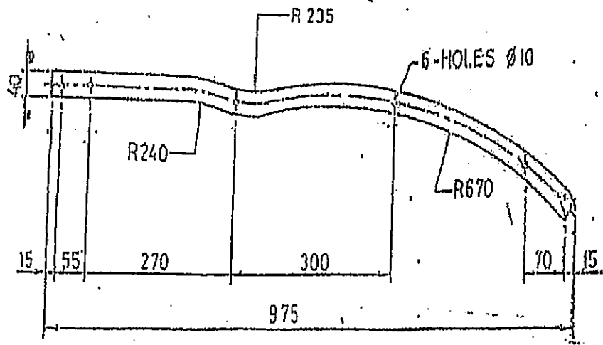
4 FRAME SCALE-1:7.5
