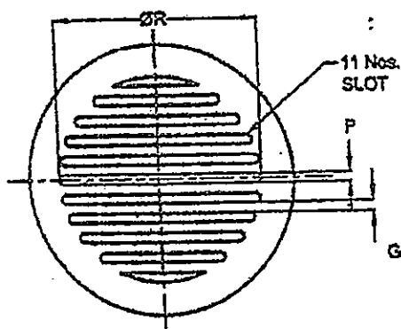
2C Grate
