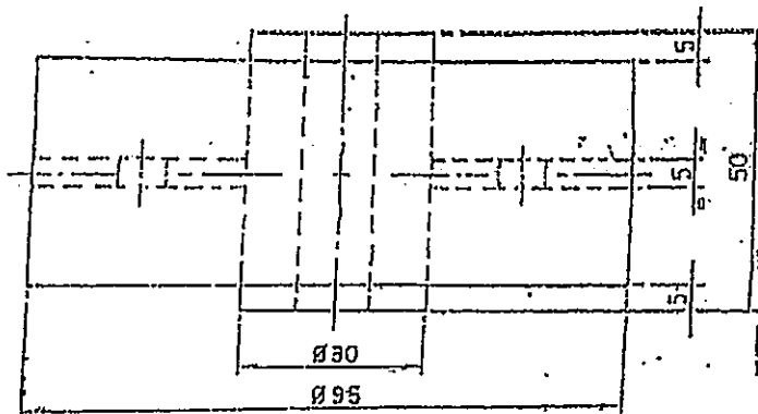
6 WHEEL (SPECIAL TYPE) SCALE 1:1
