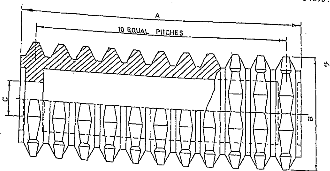
7A LOWER FEED ROLLER
