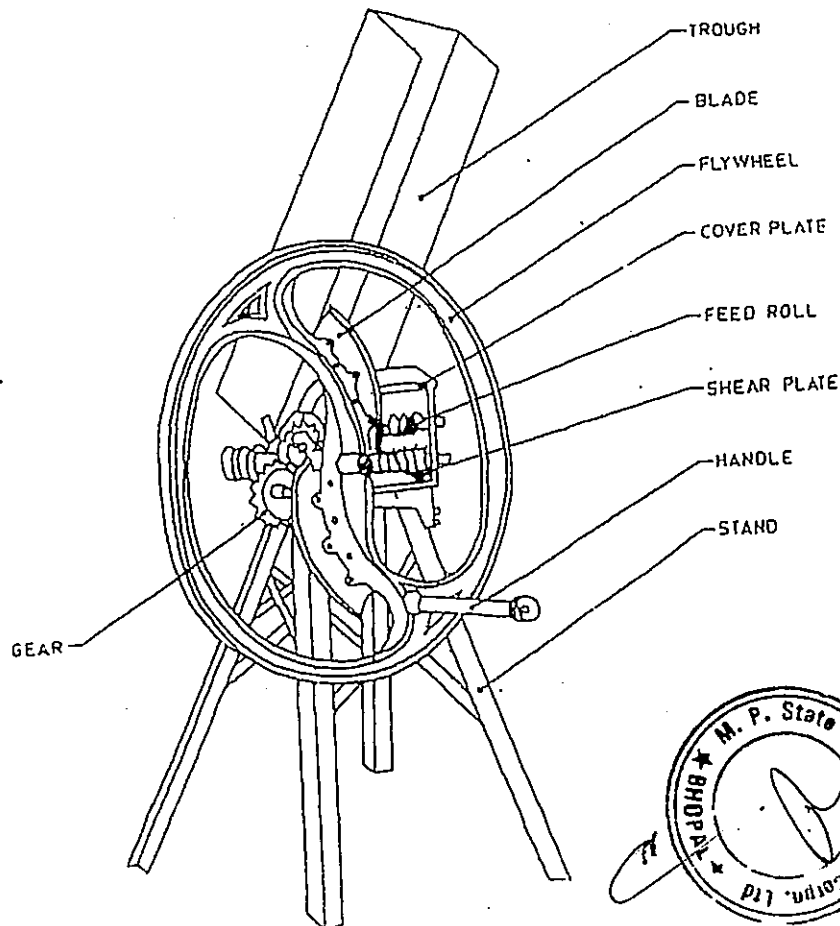
FIG. 1 Typical Drawing of Manually-Operated Chaff Cutter
