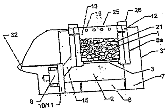
4B Solid Bio-Mass Cookstove Design 'C' without Battery
