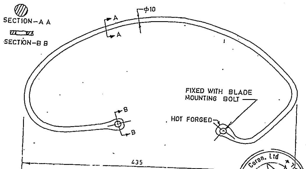
FIG. 14 FRONT SAFETY GUARD
