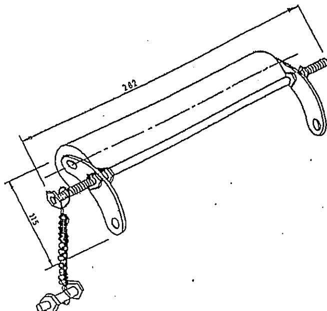
All dimensions in millimetres. FIG. 15 WARNING ROLLER
