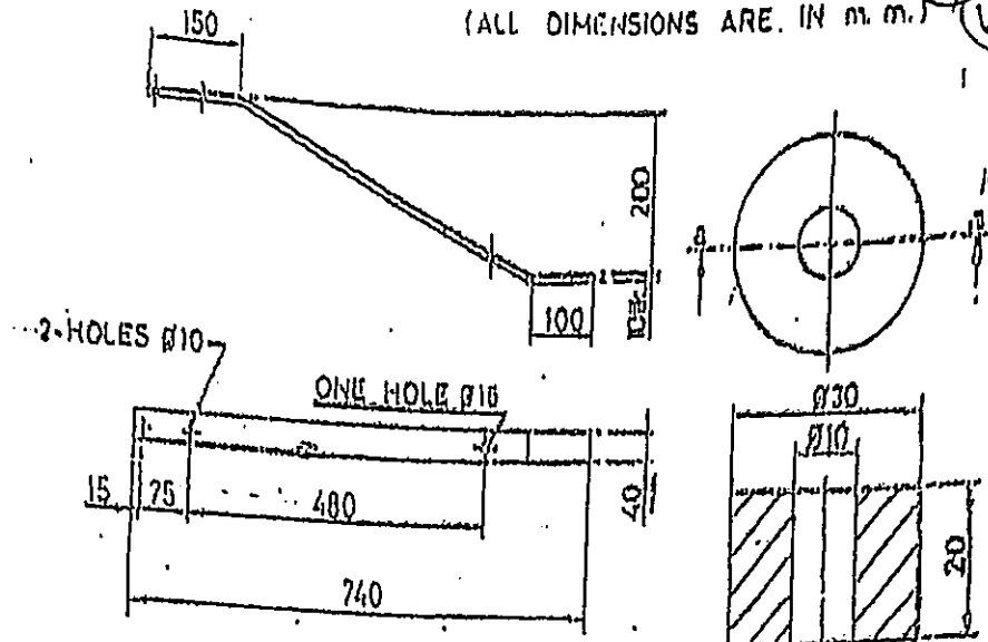
1 HANDLE SCALE-1:10
