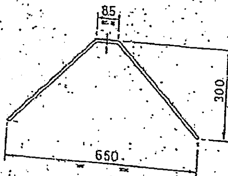
5 FRONT TYNE SUPPORT SCALE-1:10
