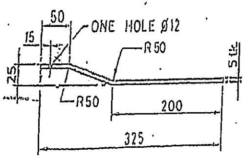
5 WHEEL BRACKET SCALE-1:5
