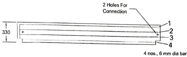
Reinforcement Plan of Top Plank (1500 mm X 330 mm)
