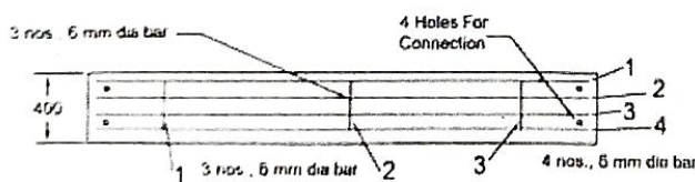
Reinforcement Plan of Bottom Plank (1360 mm X 400 mm)
