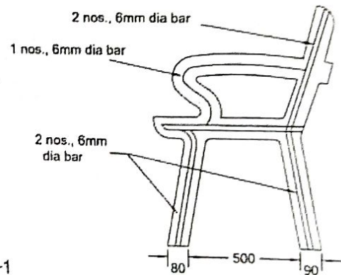
Reinforcement Detail of Leg (Isometric View)
