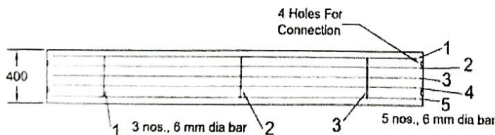
Reinforcement Plan of Bottom Plank (1510 mm X 400 mm)
