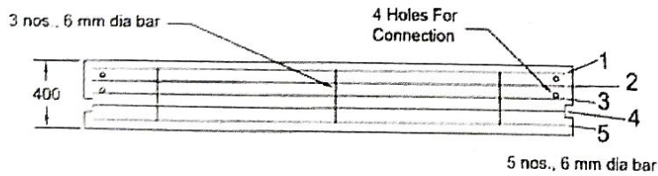
Reinforcement Plan of Bottom Plank (1500 mm X 450 mm)
