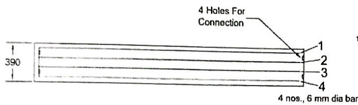
Reinforcement Plan of Top Plank (1510 mm X 390 mm)
