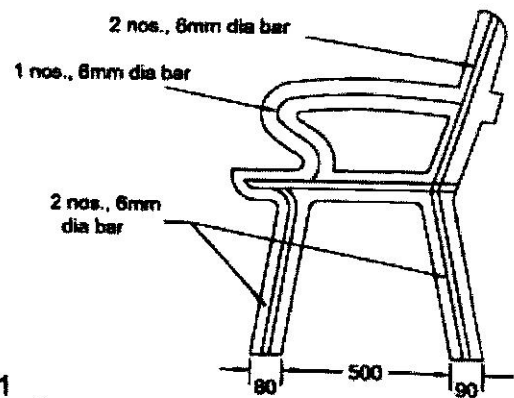
Reinforcement Detail of Leg (Isometric View)
