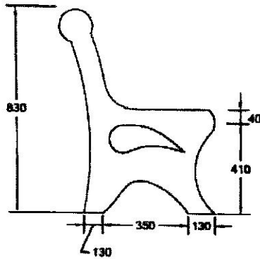
Side Elevation
