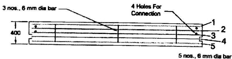
Reinforcement Plan of Bottom Plank (1500 mm X 450 mm)
