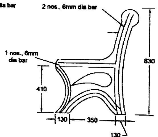
Reinforcement Detail of Leg (Isometric View)
